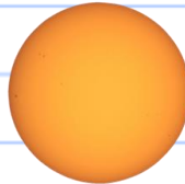
14. sunspots
