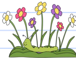
8. spring
