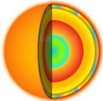
13. chromosphere
