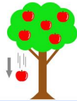
15. gravity
